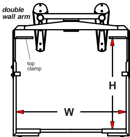
FRONT VIEW JUMBO MOUNT WALL KIT
