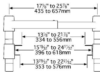
inside clearances of adjustable model
