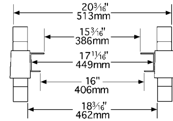
inside clearances of standard model
